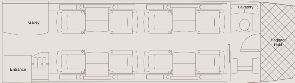
CHALLENGER 300 CABIN CONFIGURATION
